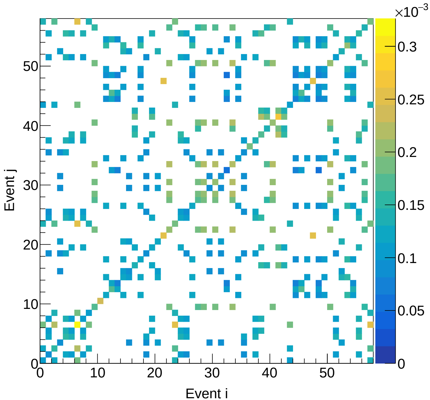
LH2 (total) Covariance | M: [6.0, 6.3) xF: [0.45, 0.50)
