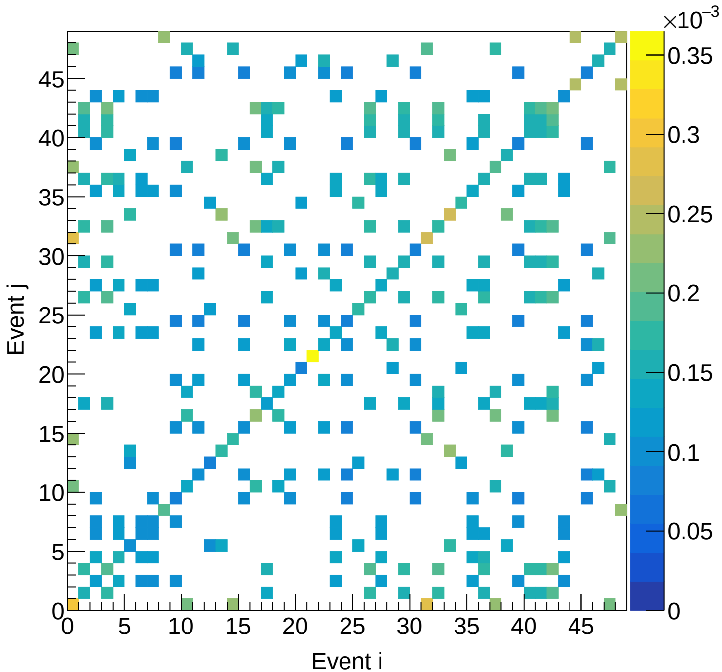
LH2 (total) Covariance | M: [6.3, 6.6] xF: [0.45, 0.50]
