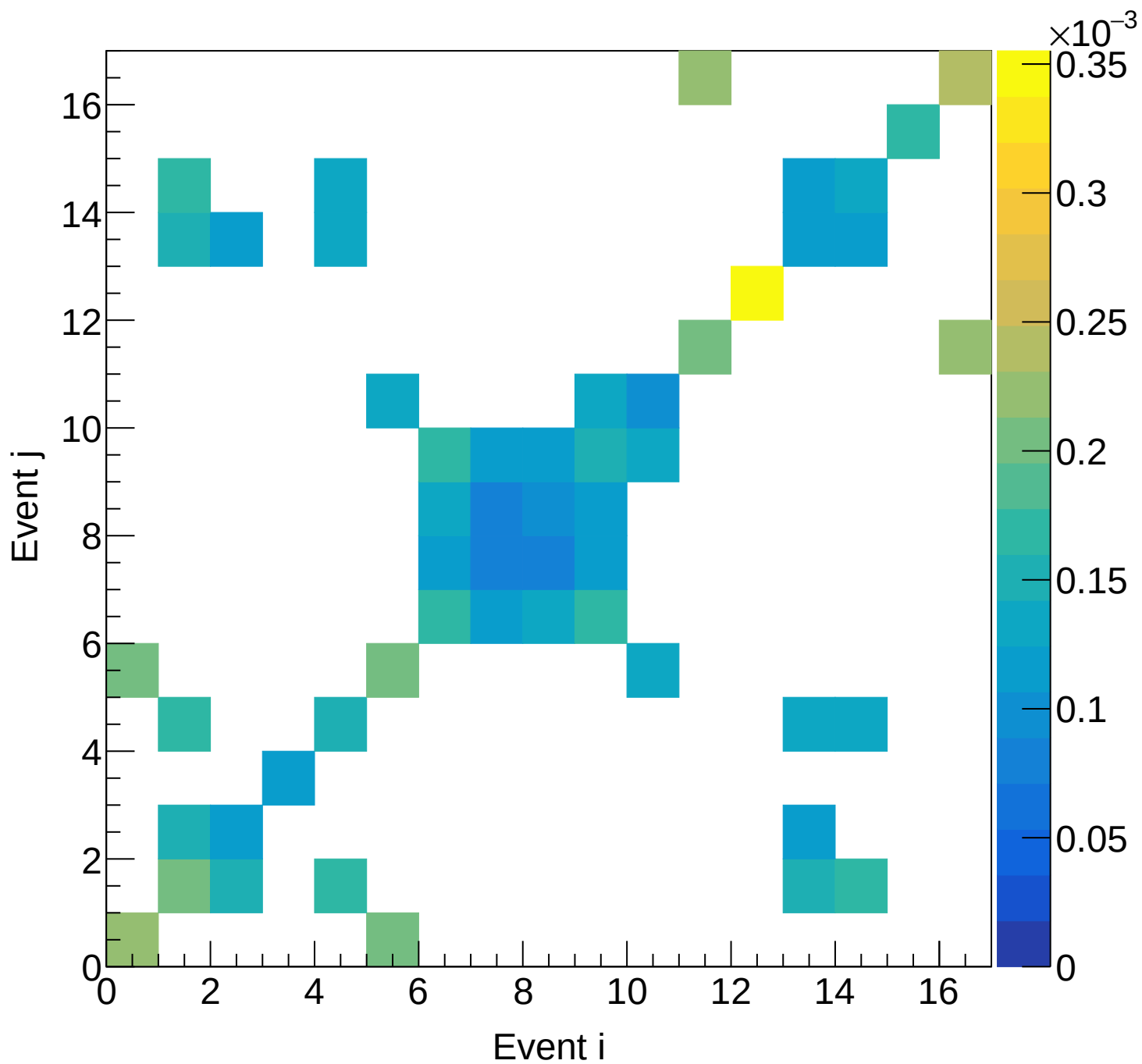
LH2 (total) Covariance | M: [6.6, 6.9] xF: [0.45, 0.50)
