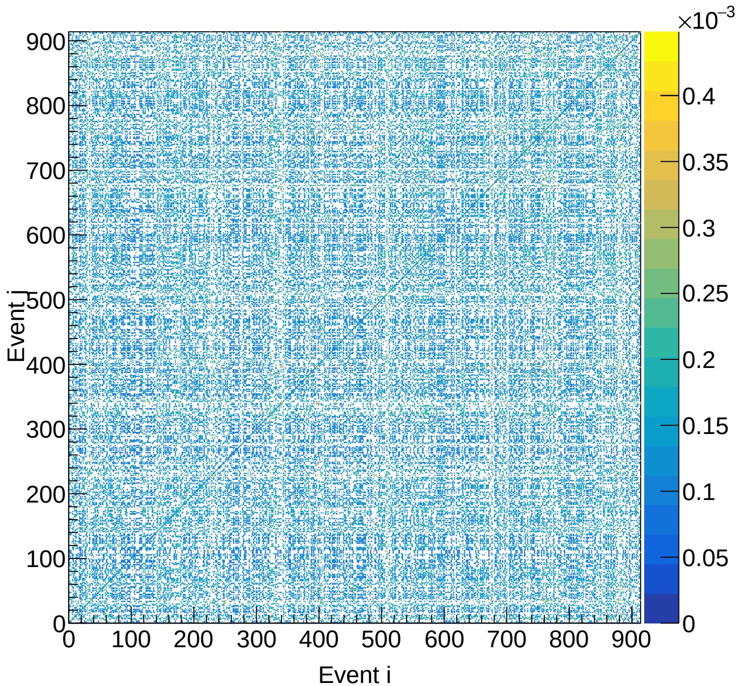
LH2 (total) Covariance | M: [3.9, 4.2) xF: [0.50, 0.55)
