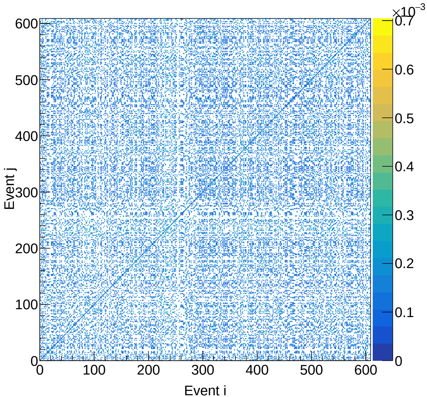
LH2 (total) Covariance | M: [4.2, 4.5) xF: [0.50, 0.55)
