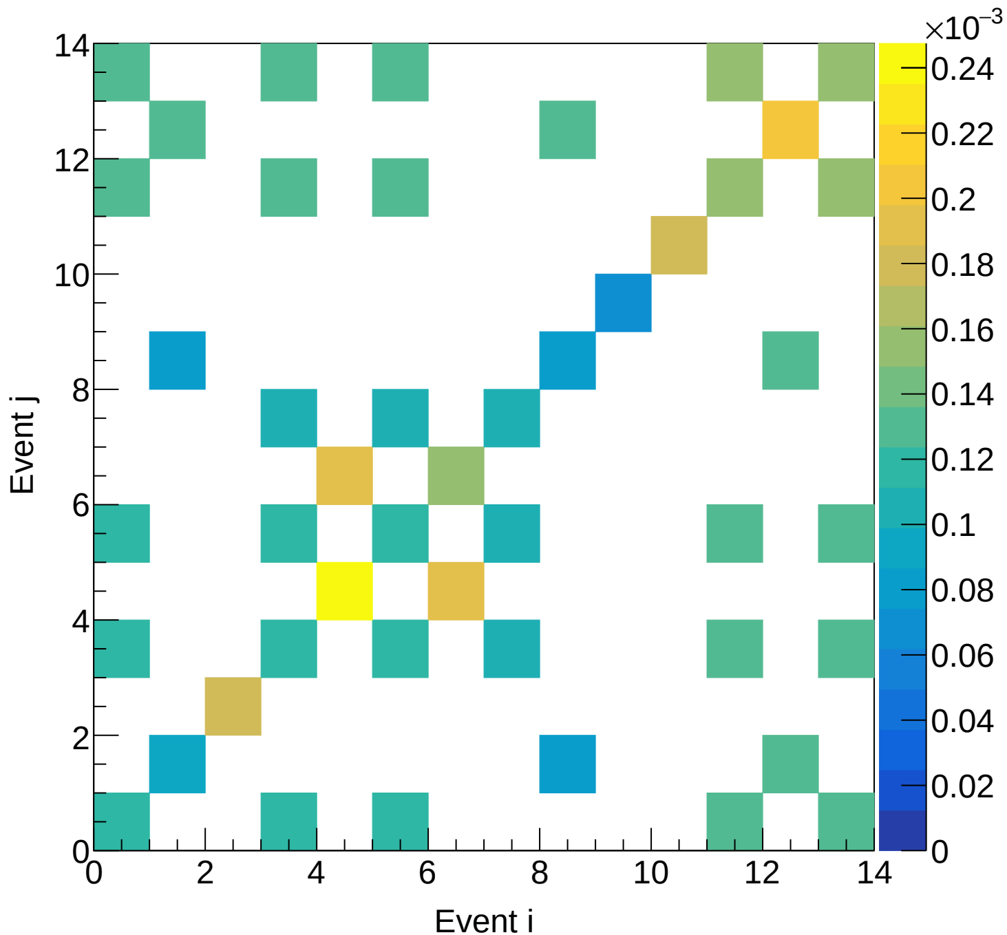
LH2 (total) Covariance | M: [6.9, 7.5) xF: [0.50, 0.55)
