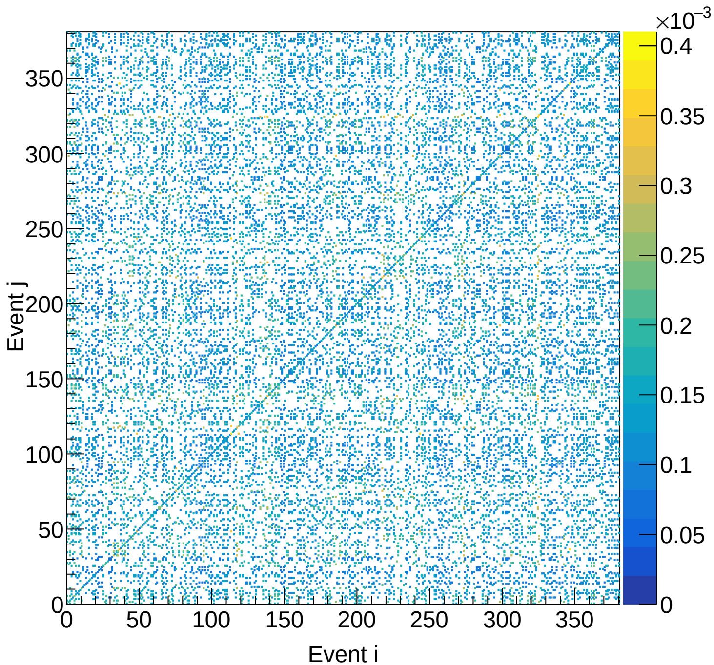
LH2 (total) Covariance | M: [4.5, 4.8) xF: [0.50, 0.55)
