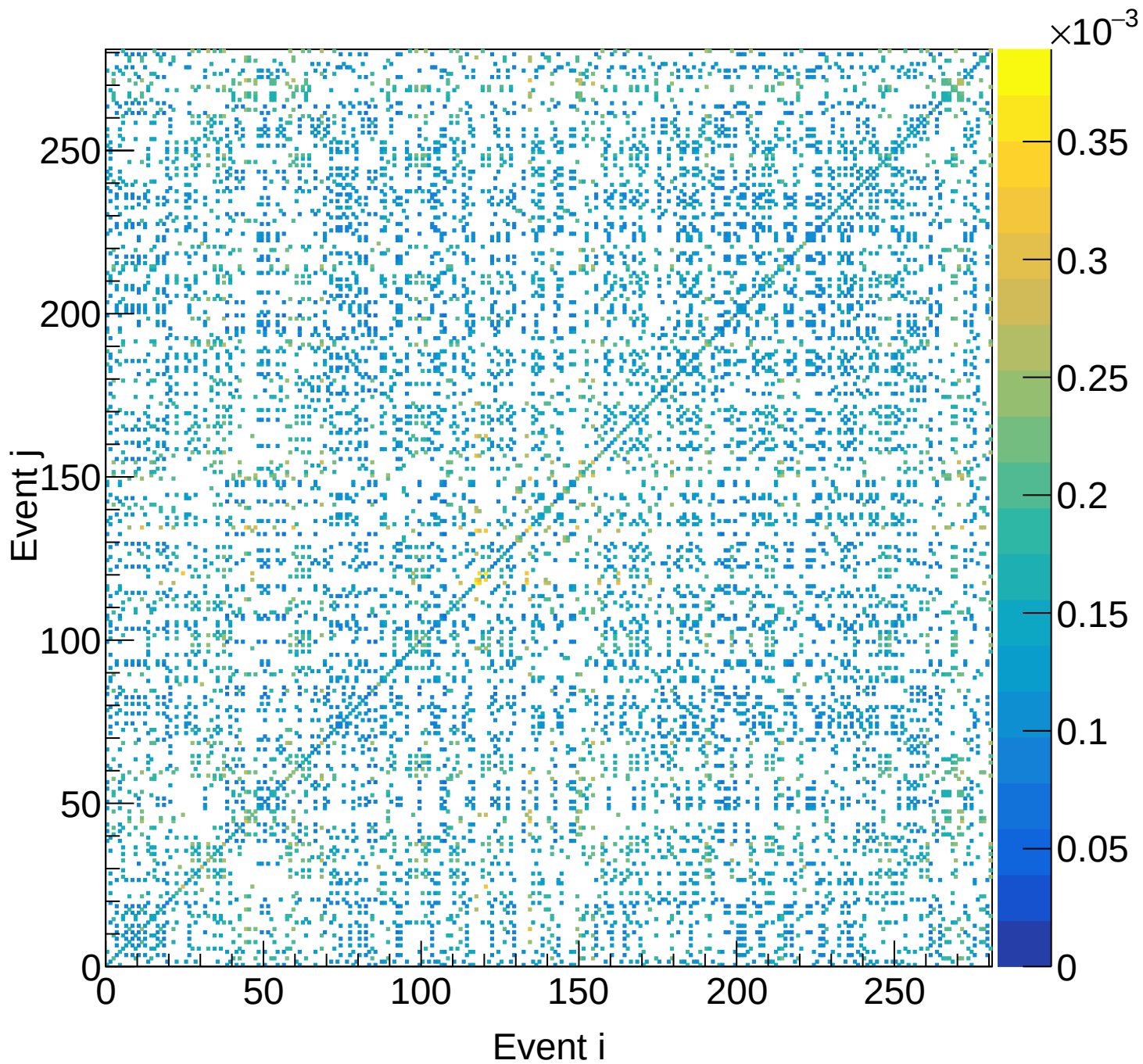
LH2 (total) Covariance | M: [4.8, 5.1) xF: [0.50, 0.55)
