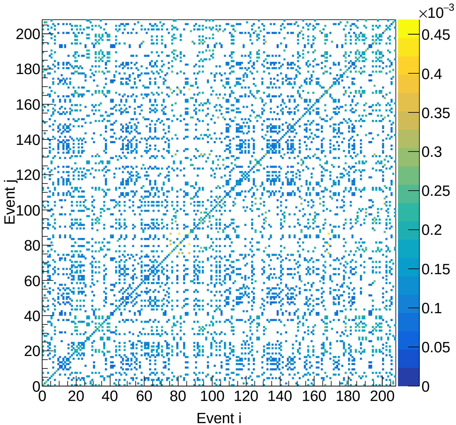
LH2 (total) Covariance | M: [5.1, 5.4) xF: [0.50, 0.55)
