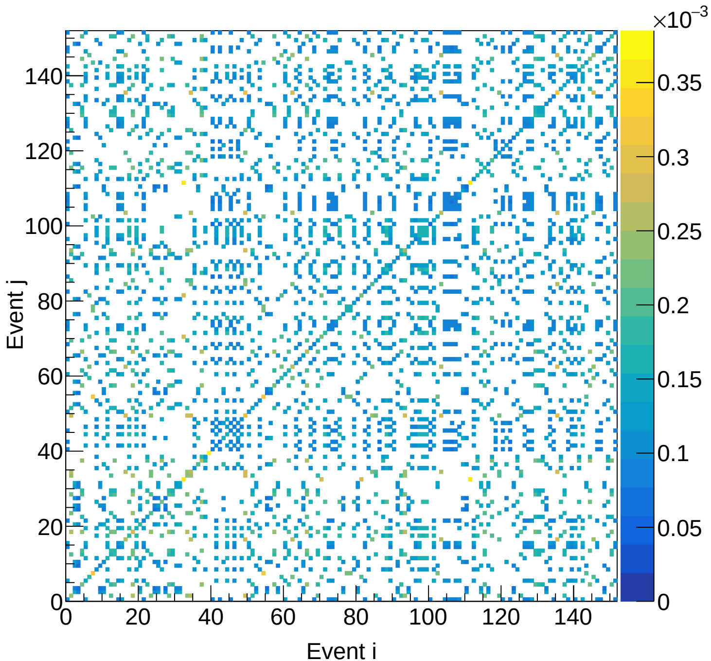
LH2 (total) Covariance | M: [5.4, 5.7) xF: [0.50, 0.55)
