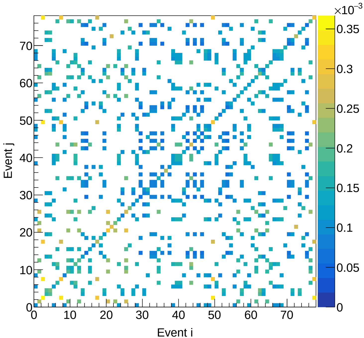
LH2 (total) Covariance | M: [5.7, 6.0) xF: [0.50, 0.55)
