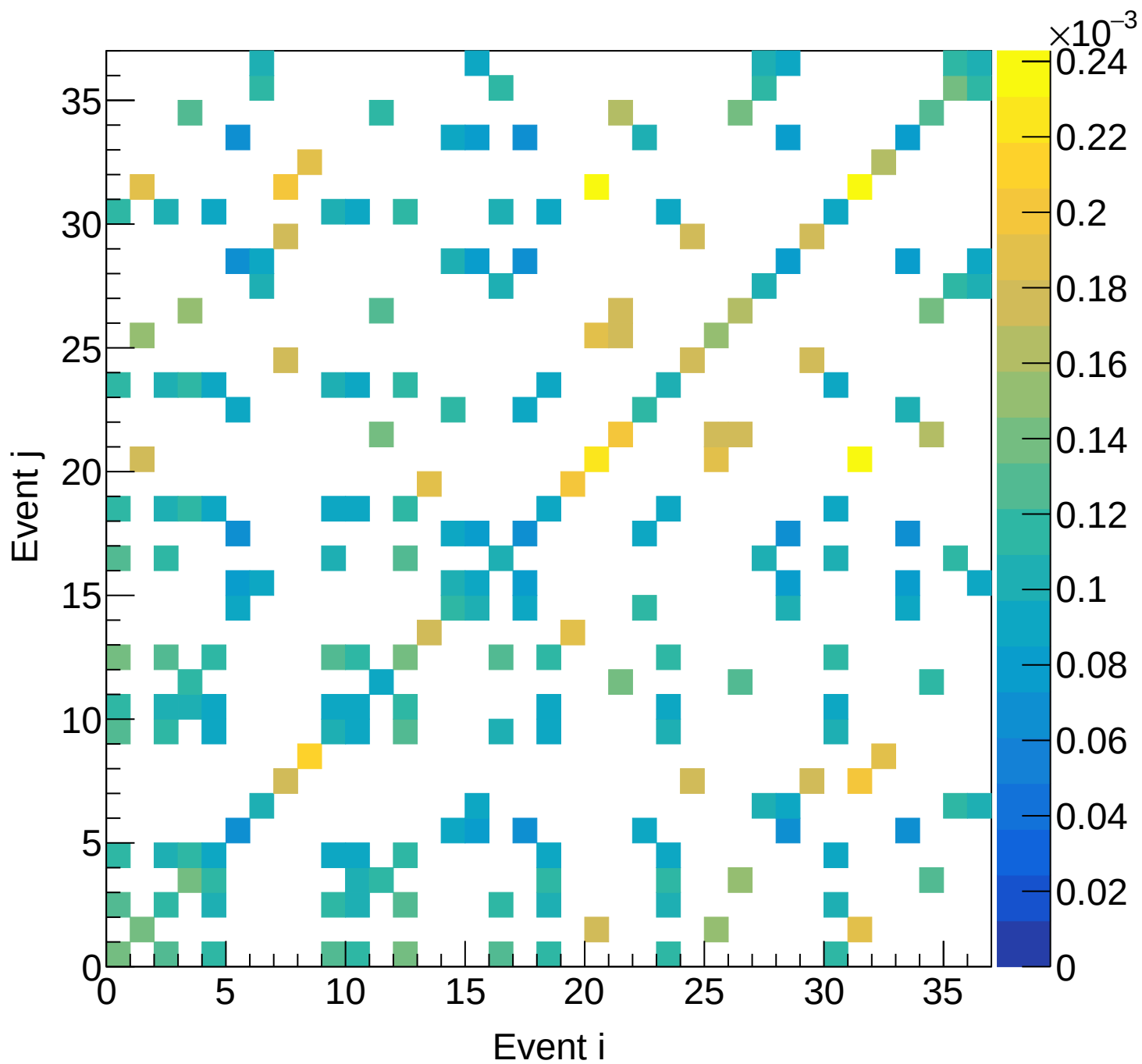
LH2 (total) Covariance | M: [6.3, 6.6) xF: [0.50, 0.55)
