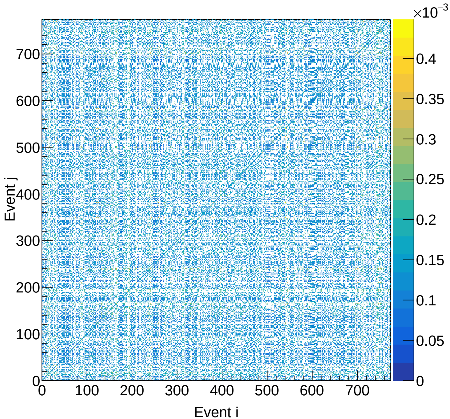
LH2 (total) Covariance | M: [3.9, 4.2) xF: [0.55, 0.60)
