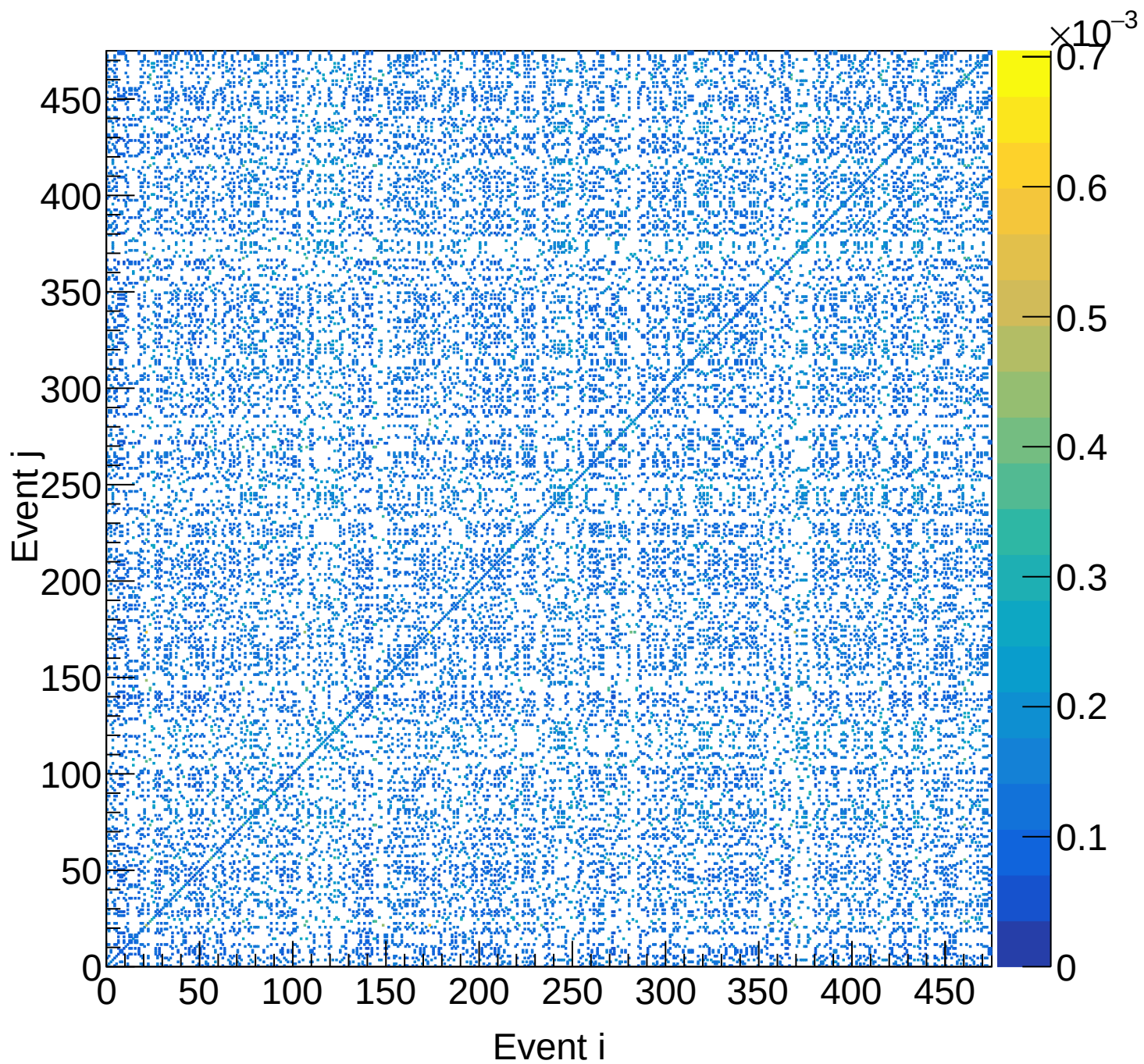
LH2 (total) Covariance | M: [4.2, 4.5) xF: [0.55, 0.60)
