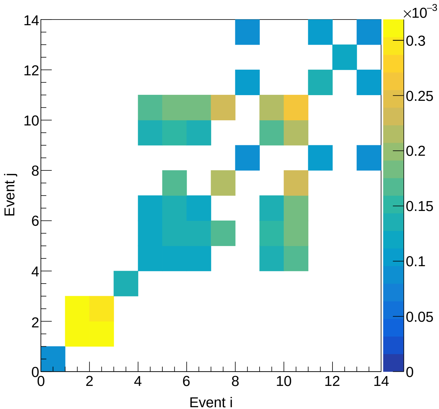
LH2 (total) Covariance | M: [6.9, 7.5) xF: [0.55, 0.60)
