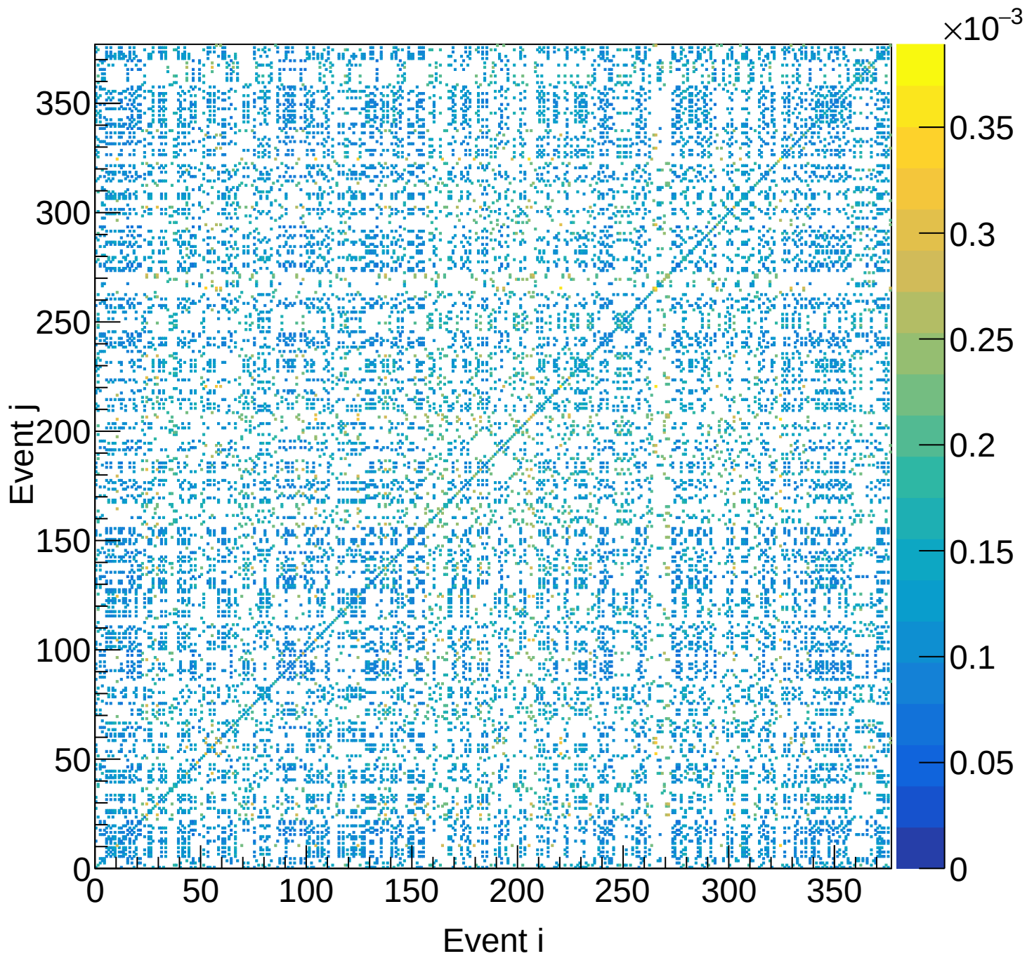
LH2 (total) Covariance | M: [4.5, 4.8) xF: [0.55, 0.60)
