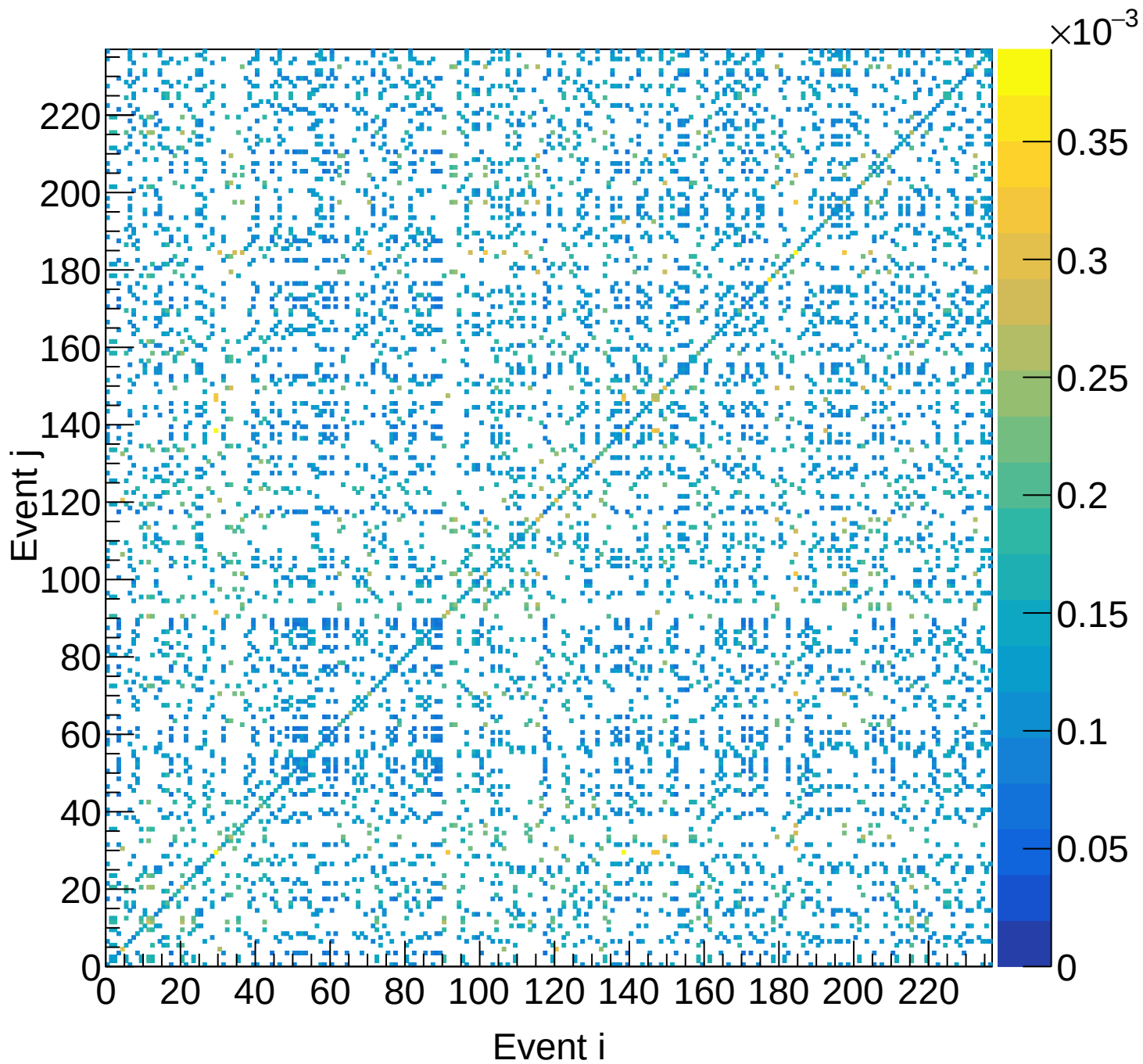
LH2 (total) Covariance | M: [4.8, 5.1) xF: [0.55, 0.60)
