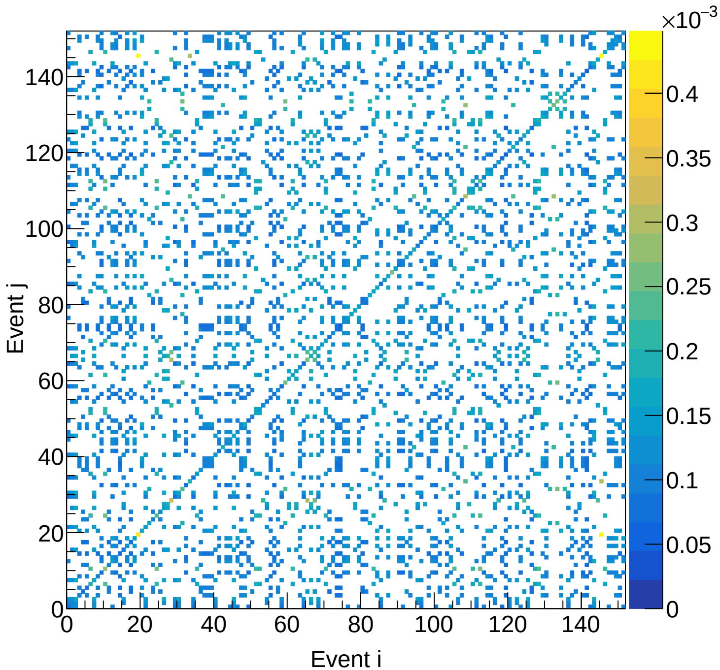
LH2 (total) Covariance | M: [5.1, 5.4) xF: [0.55, 0.60)
