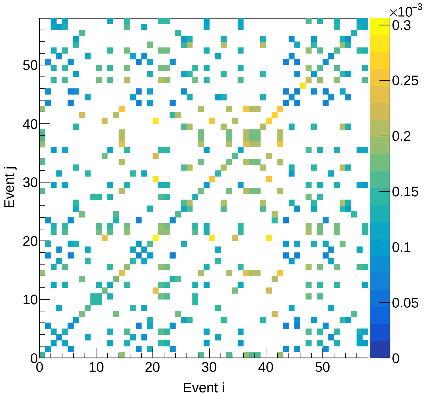
LH2 (total) Covariance | M: [5.7, 6.0] xF: [0.55, 0.60]
