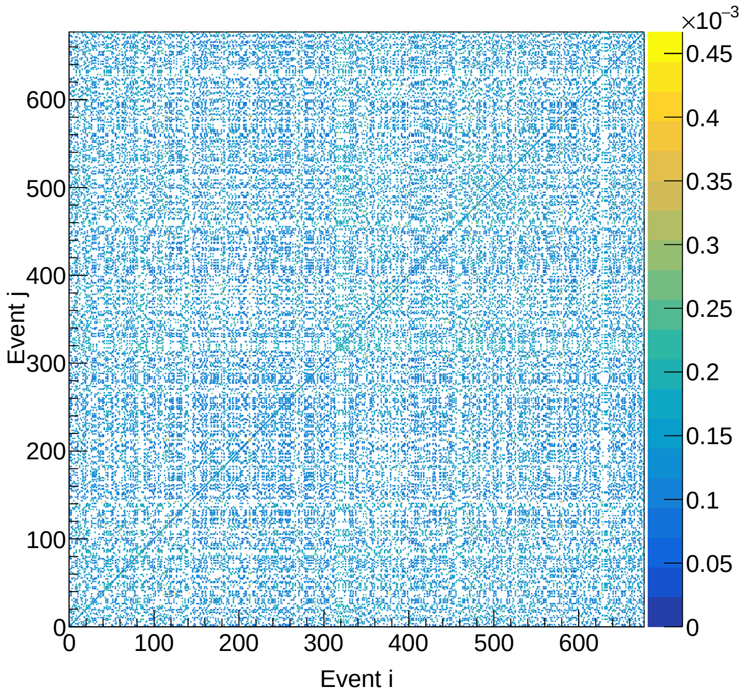
LH2 (total) Covariance | M: [3.9, 4.2) xF: [0.60, 0.65)
