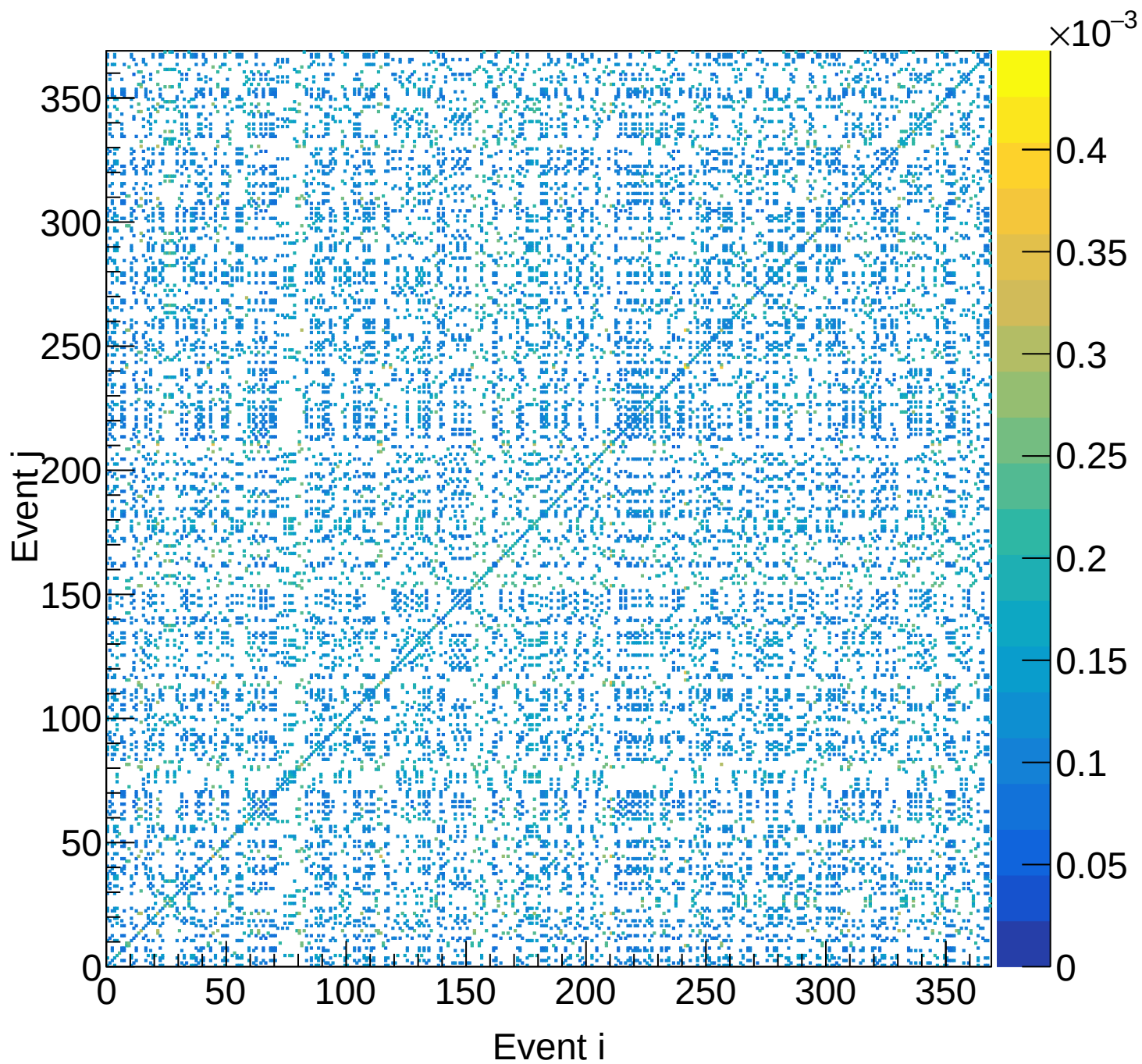
LH2 (total) Covariance | M: [4.2, 4.5) xF: [0.60, 0.65)
