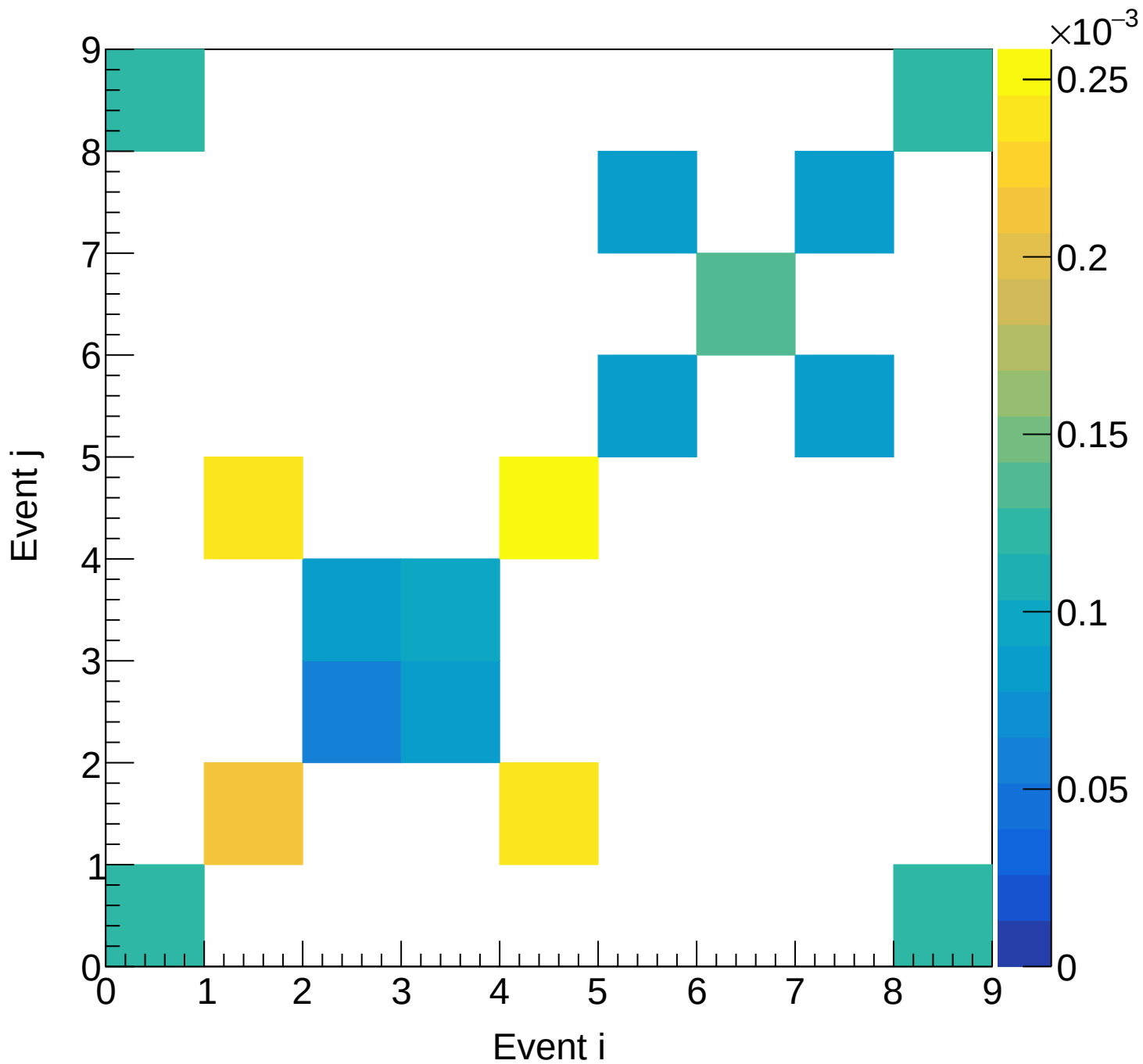
LH2 (total) Covariance | M: [6.9, 7.5] xF: [0.60, 0.65]
