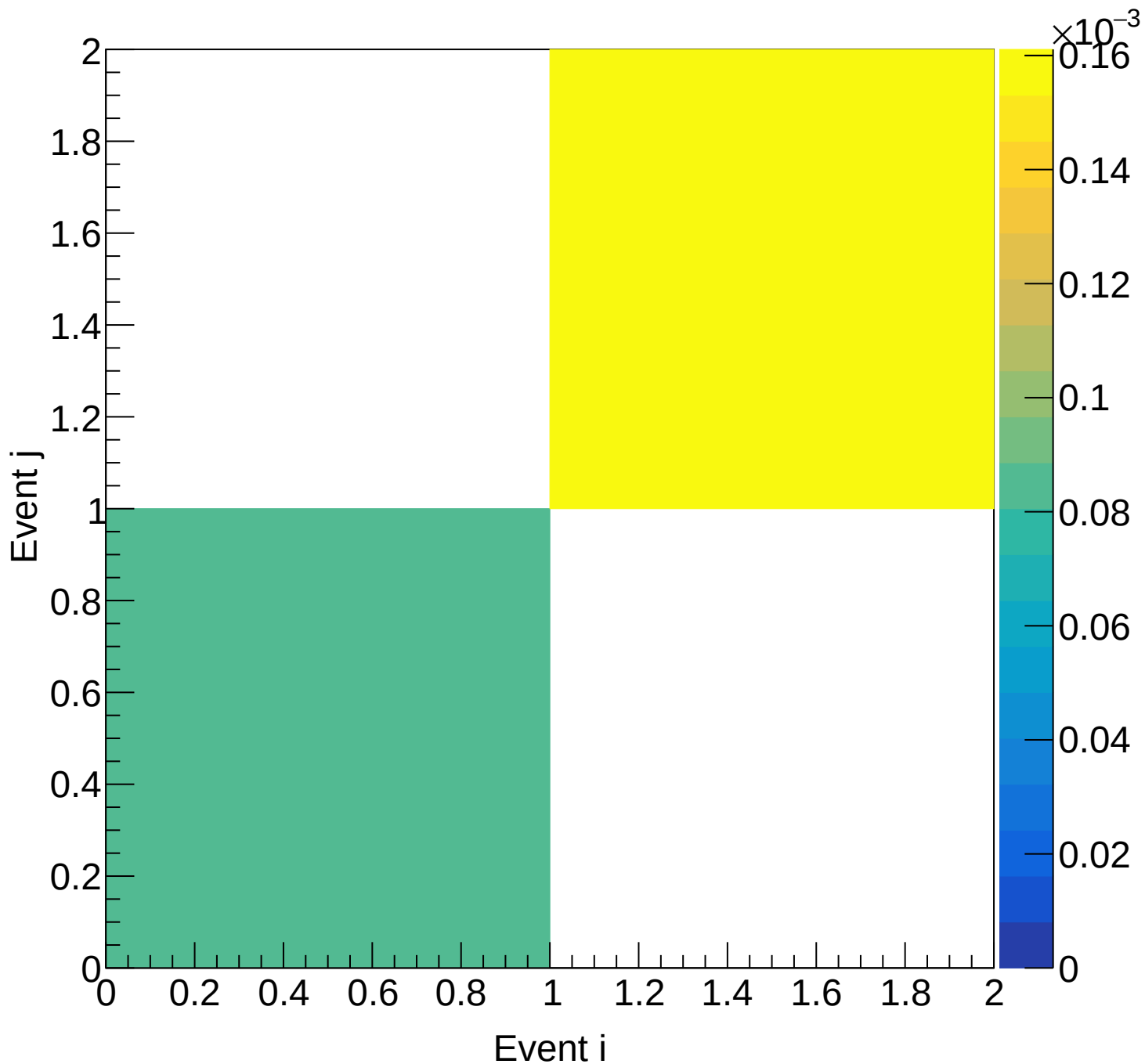
LH2 (total) Covariance | M: [7.5, 8.8) xF: [0.60, 0.65)
