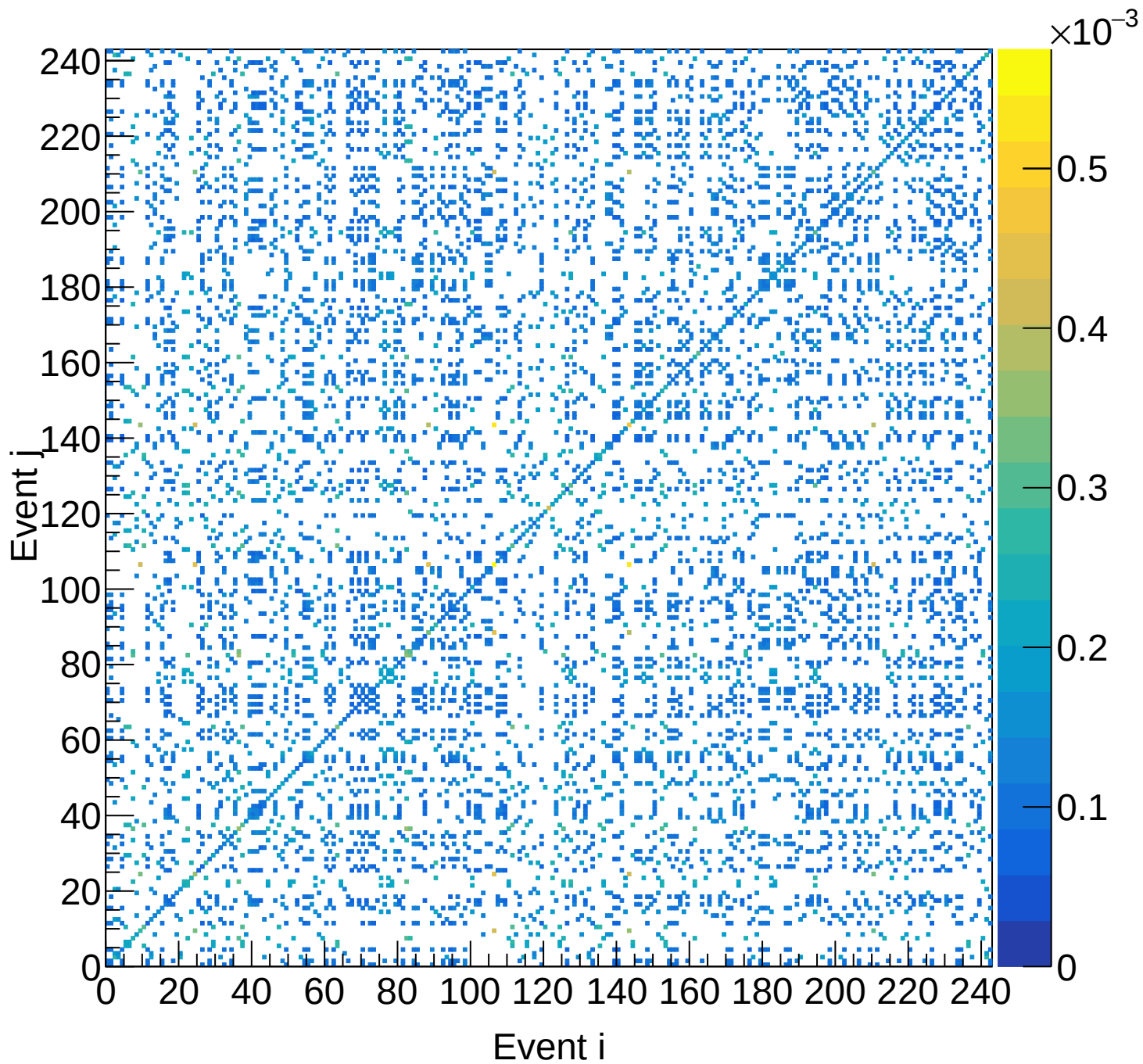
LH2 (total) Covariance | M: [4.5, 4.8) xF: [0.60, 0.65)
