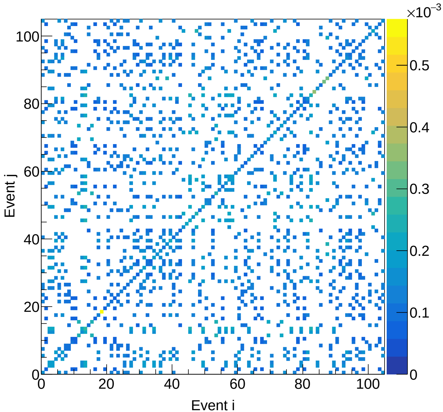
LH2 (total) Covariance | M: [5.1, 5.4) xF: [0.60, 0.65)
