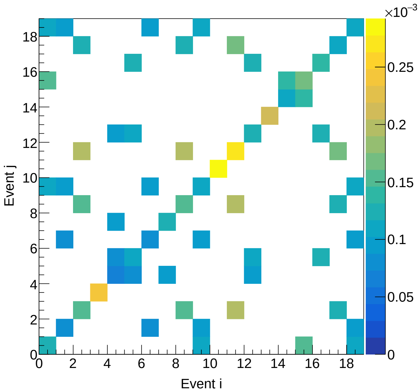
LH2 (total) Covariance | M: [6.3, 6.6) xF: [0.60, 0.65)
