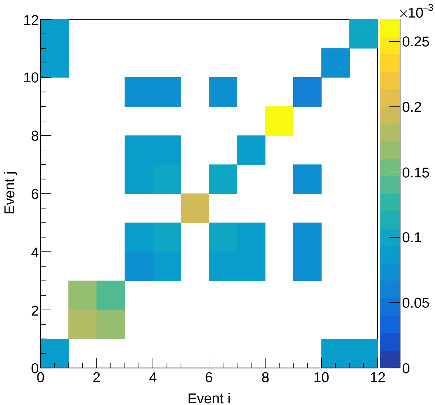
LH2 (total) Covariance | M: [6.6, 6.9) xF: [0.60, 0.65)
