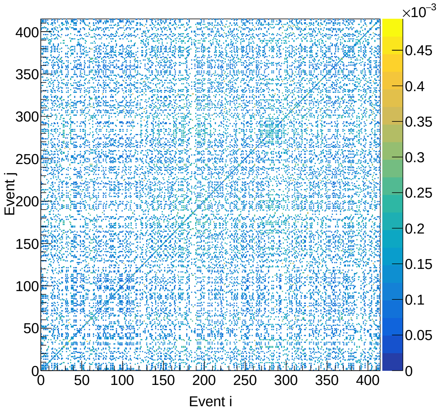
LH2 (total) Covariance | M: [3.9, 4.2) xF: [0.65, 0.70)
