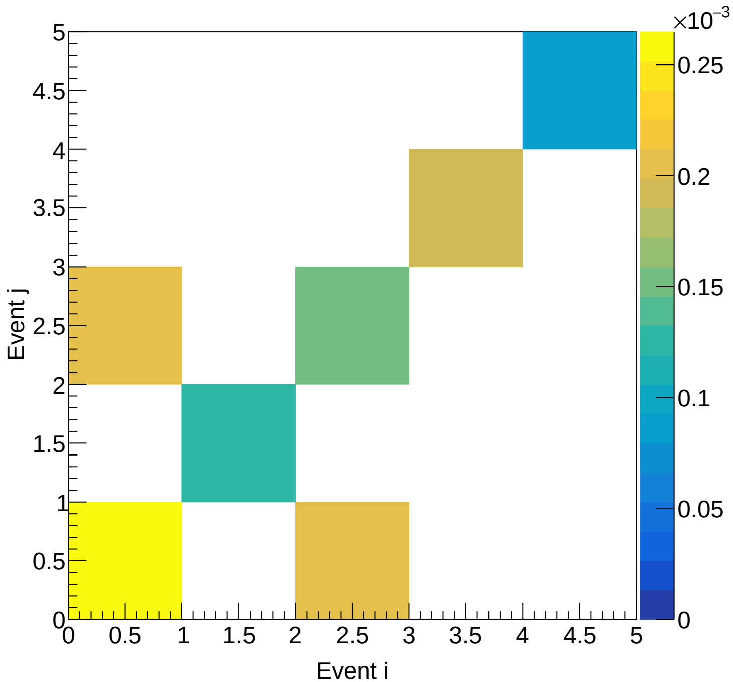
LH2 (total) Covariance | M: [7.5, 8.8) xF: [0.65, 0.70)
