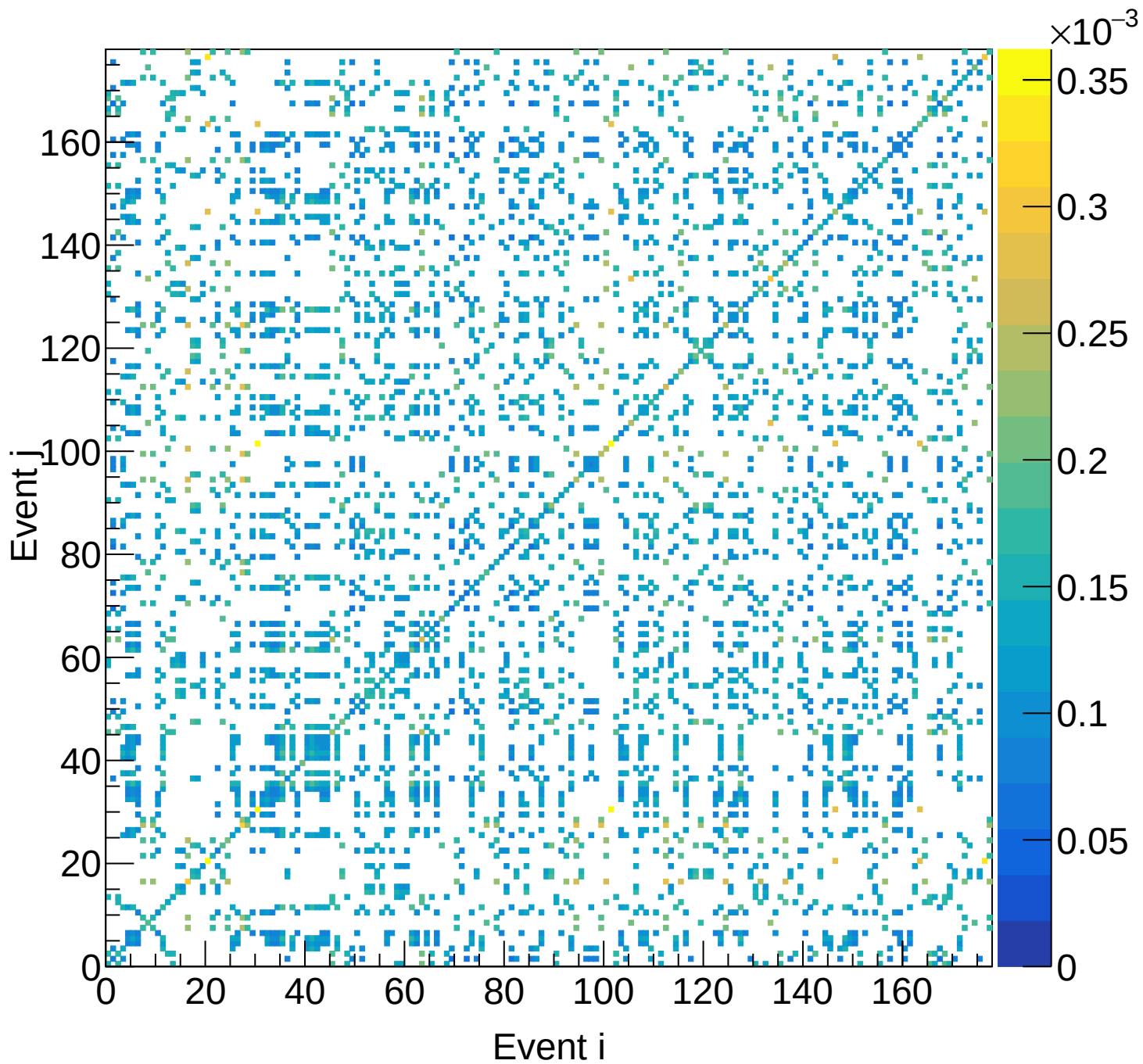
LH2 (total) Covariance | M: [4.5, 4.8) xF: [0.65, 0.70)
