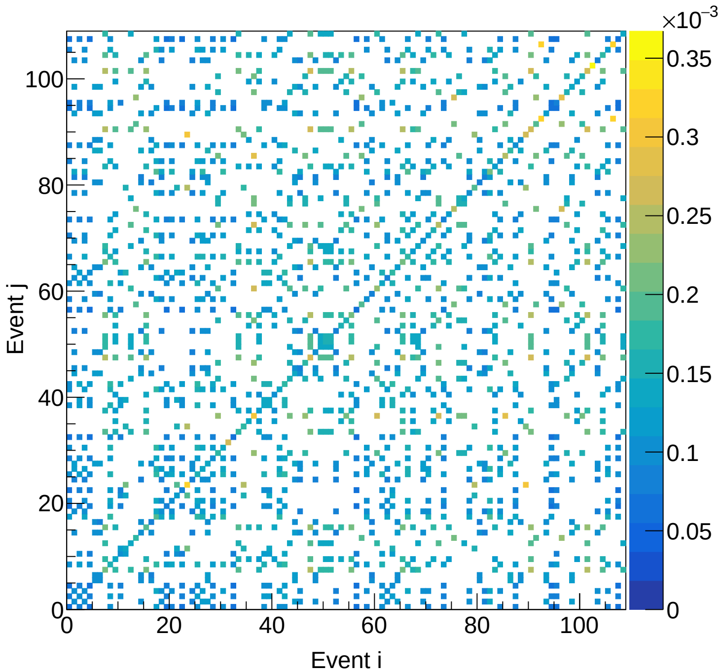
LH2 (total) Covariance | M: [4.8, 5.1) xF: [0.65, 0.70)
