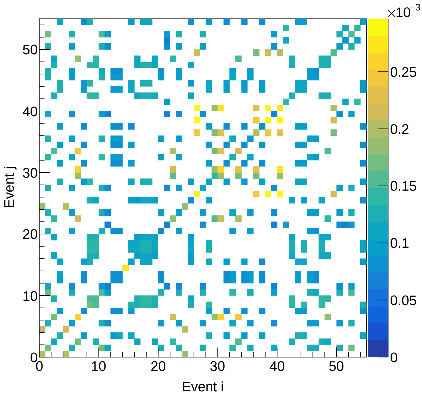
LH2 (total) Covariance | M: [5.4, 5.7) xF: [0.65, 0.70)
