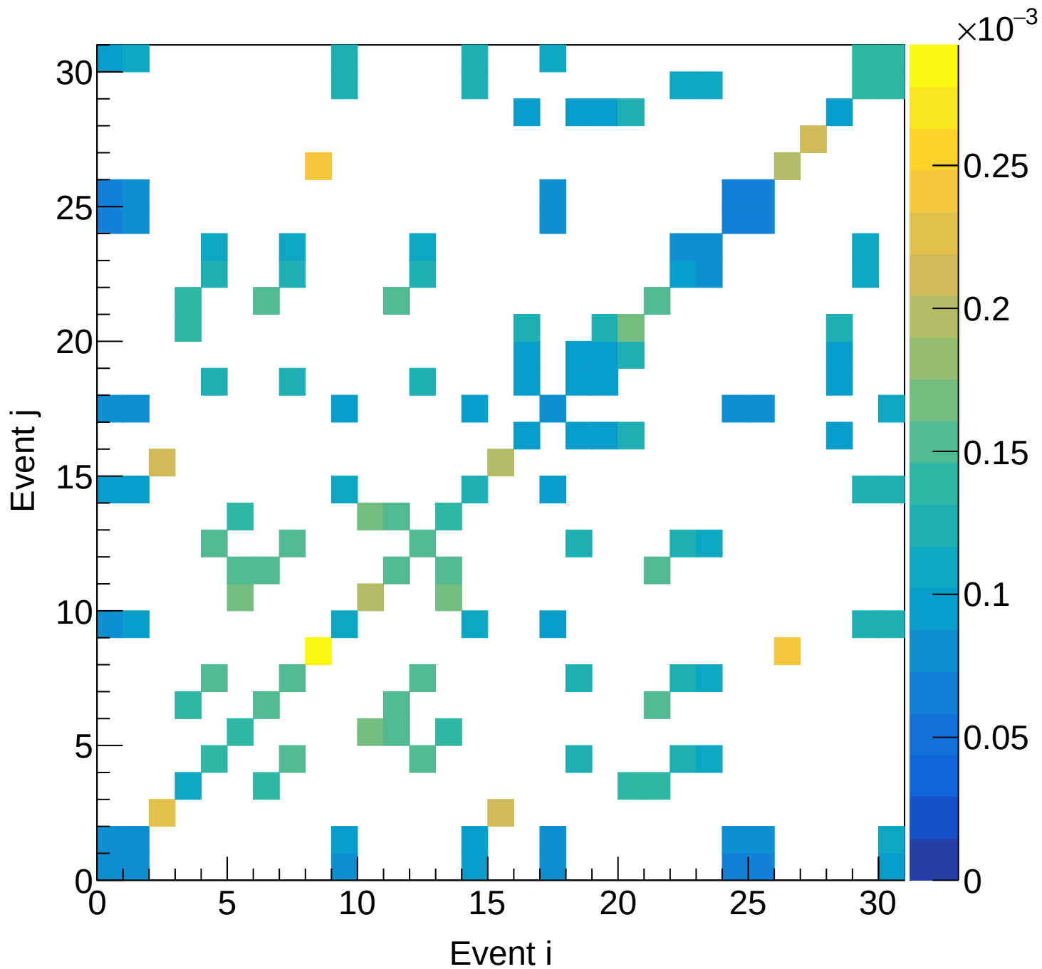
LH2 (total) Covariance | M: [5.7, 6.0] xF: [0.65, 0.70]
