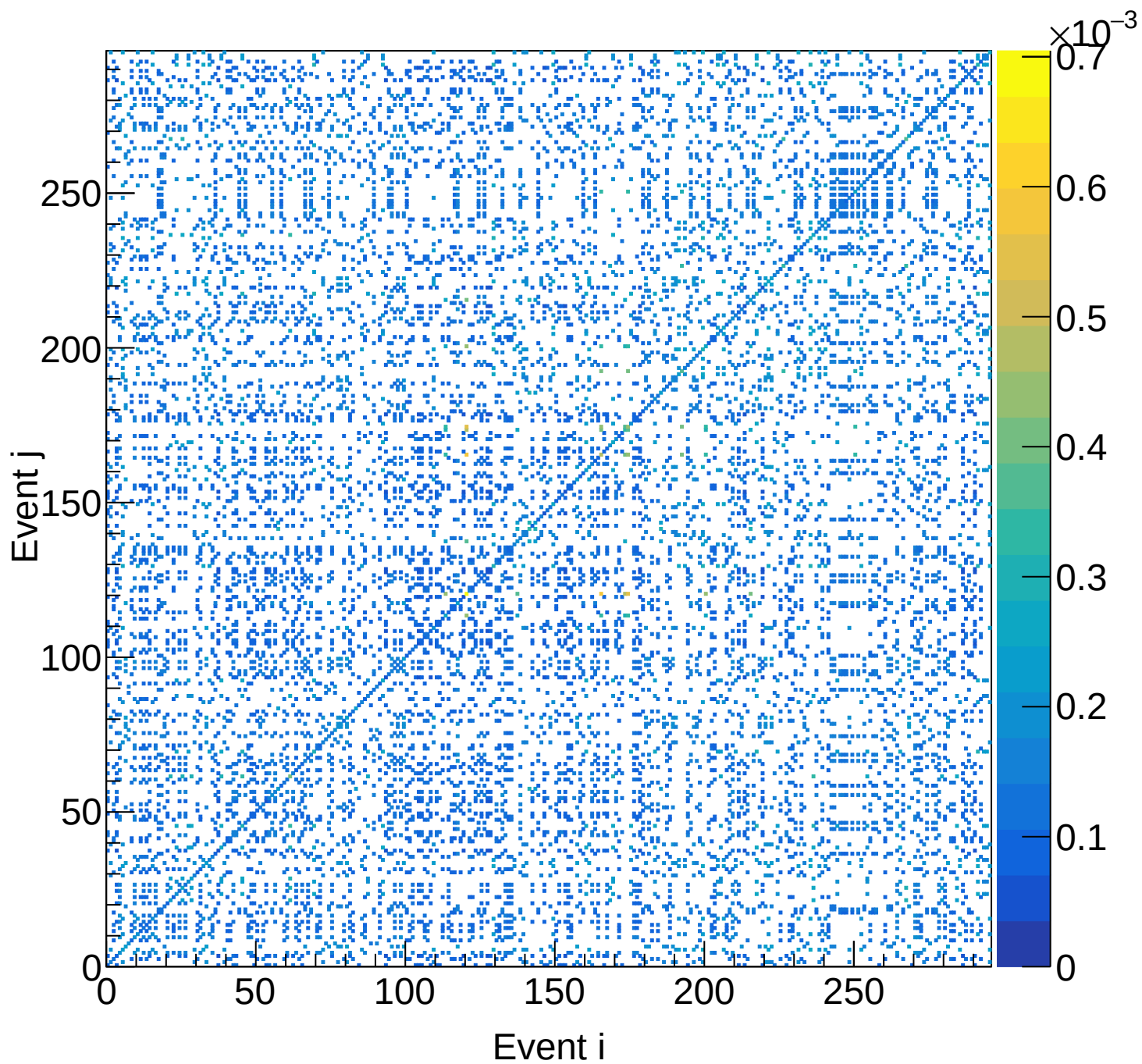
LH2 (total) Covariance | M: [3.9, 4.2) xF: [0.70, 0.75)
