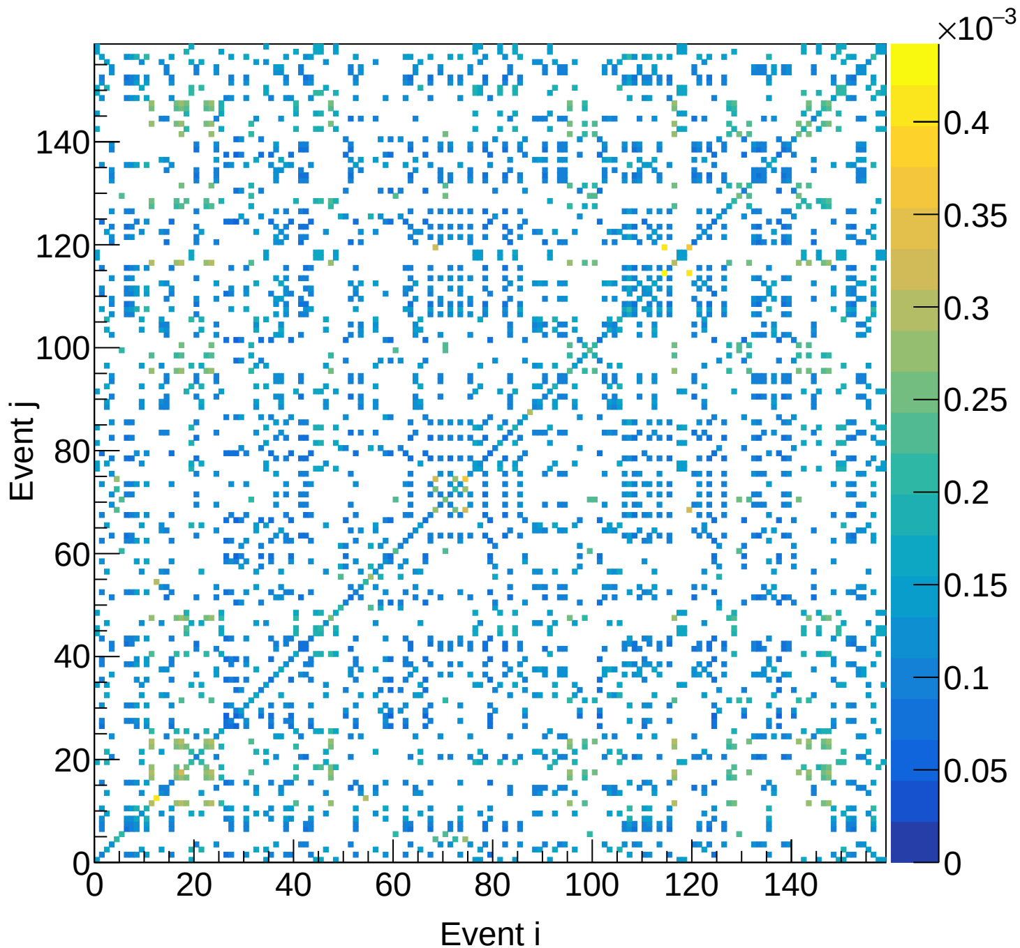
LH2 (total) Covariance | M: [4.2, 4.5) xF: [0.70, 0.75)
