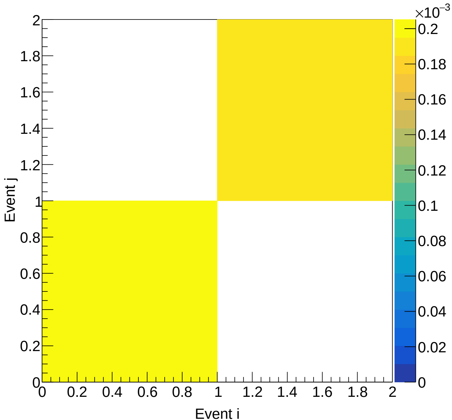
LH2 (total) Covariance | M: [7.5, 8.8) xF: [0.70, 0.75)
