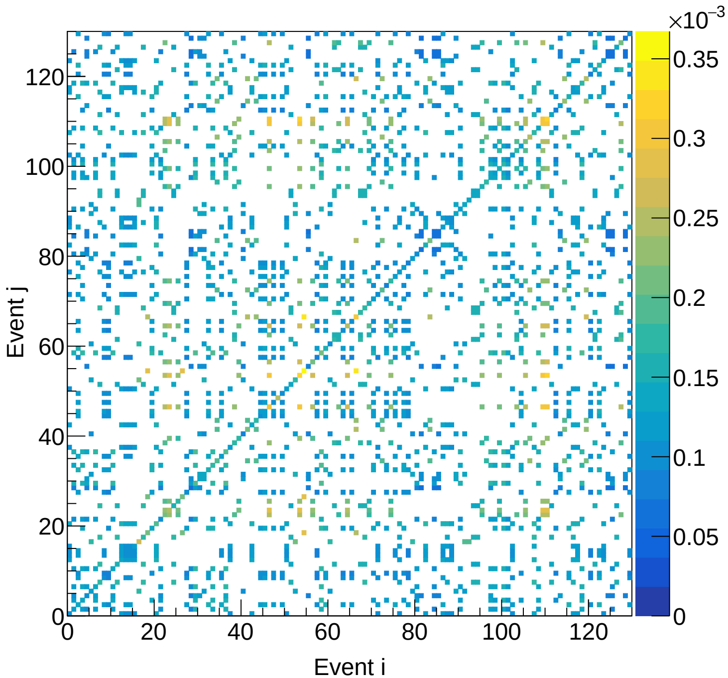
LH2 (total) Covariance | M: [4.5, 4.8) xF: [0.70, 0.75)
