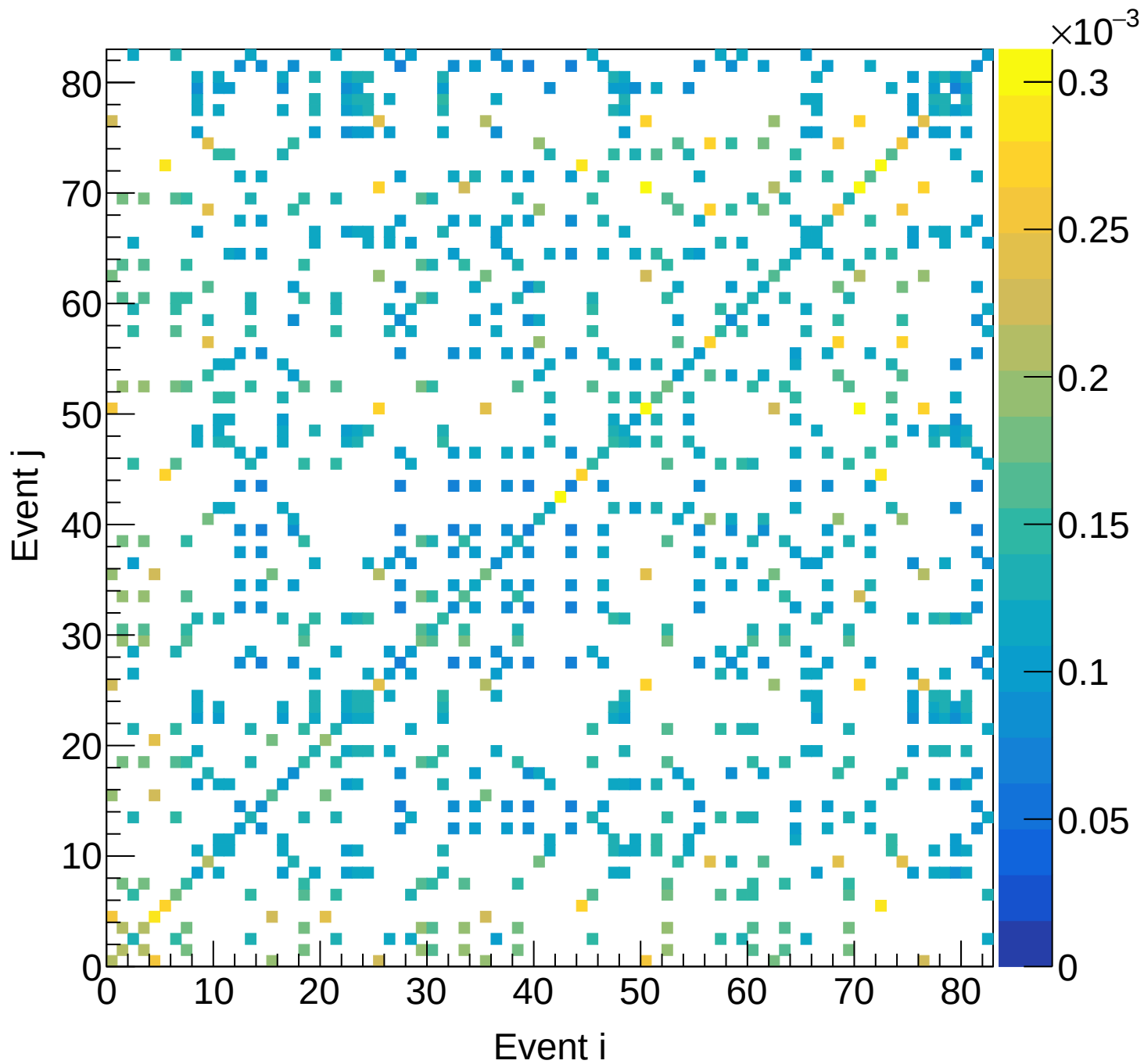
LH2 (total) Covariance | M: [4.8, 5.1) xF: [0.70, 0.75)
