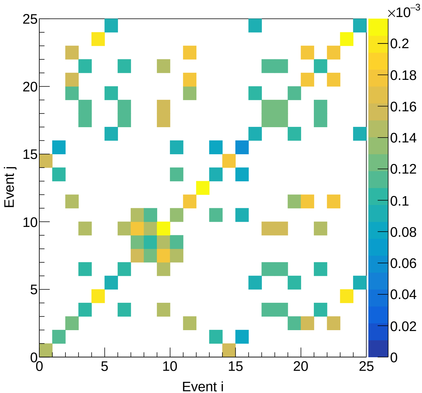
LH2 (total) Covariance | M: [5.4, 5.7) xF: [0.70, 0.75)
