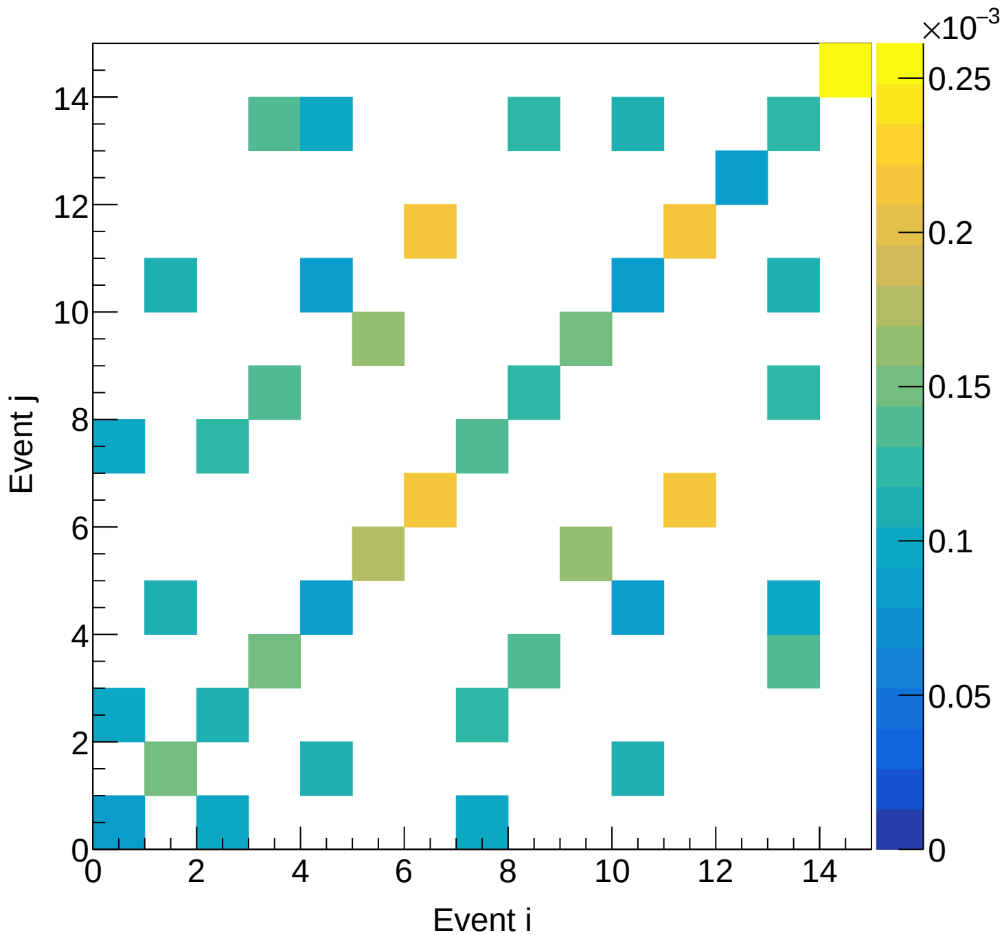
LH2 (total) Covariance | M: [6.0, 6.3) xF: [0.70, 0.75)
