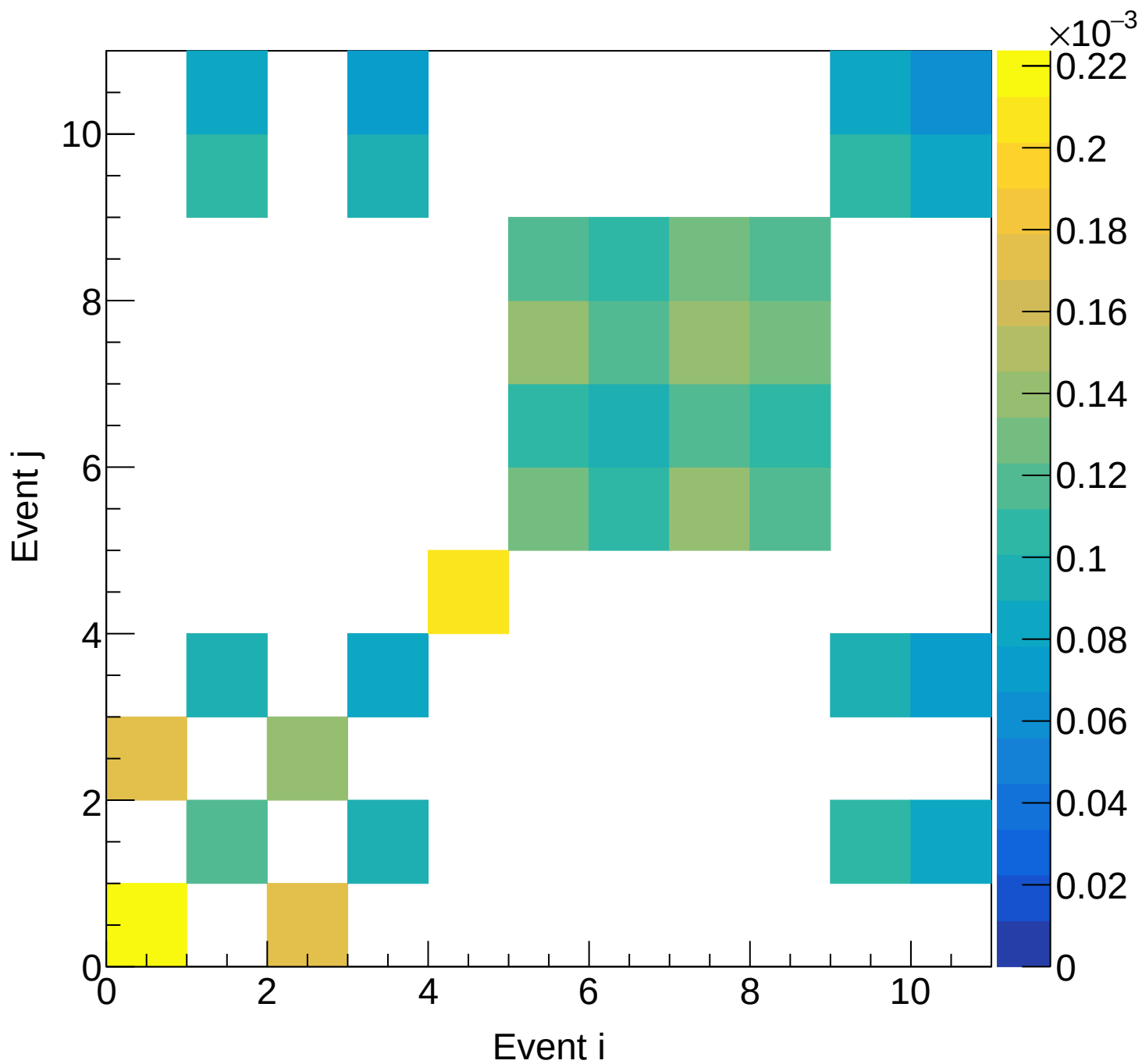
LH2 (total) Covariance | M: [6.3, 6.6) xF: [0.70, 0.75)
