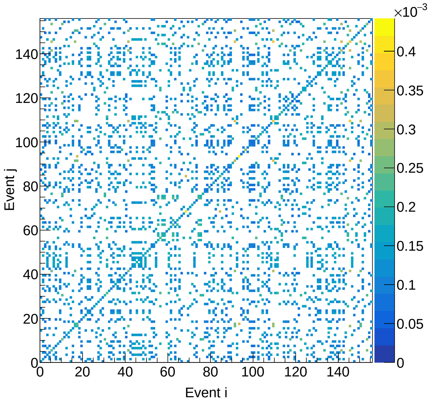
LH2 (total) Covariance | M: [3.9, 4.2) xF: [0.75, 0.80)
