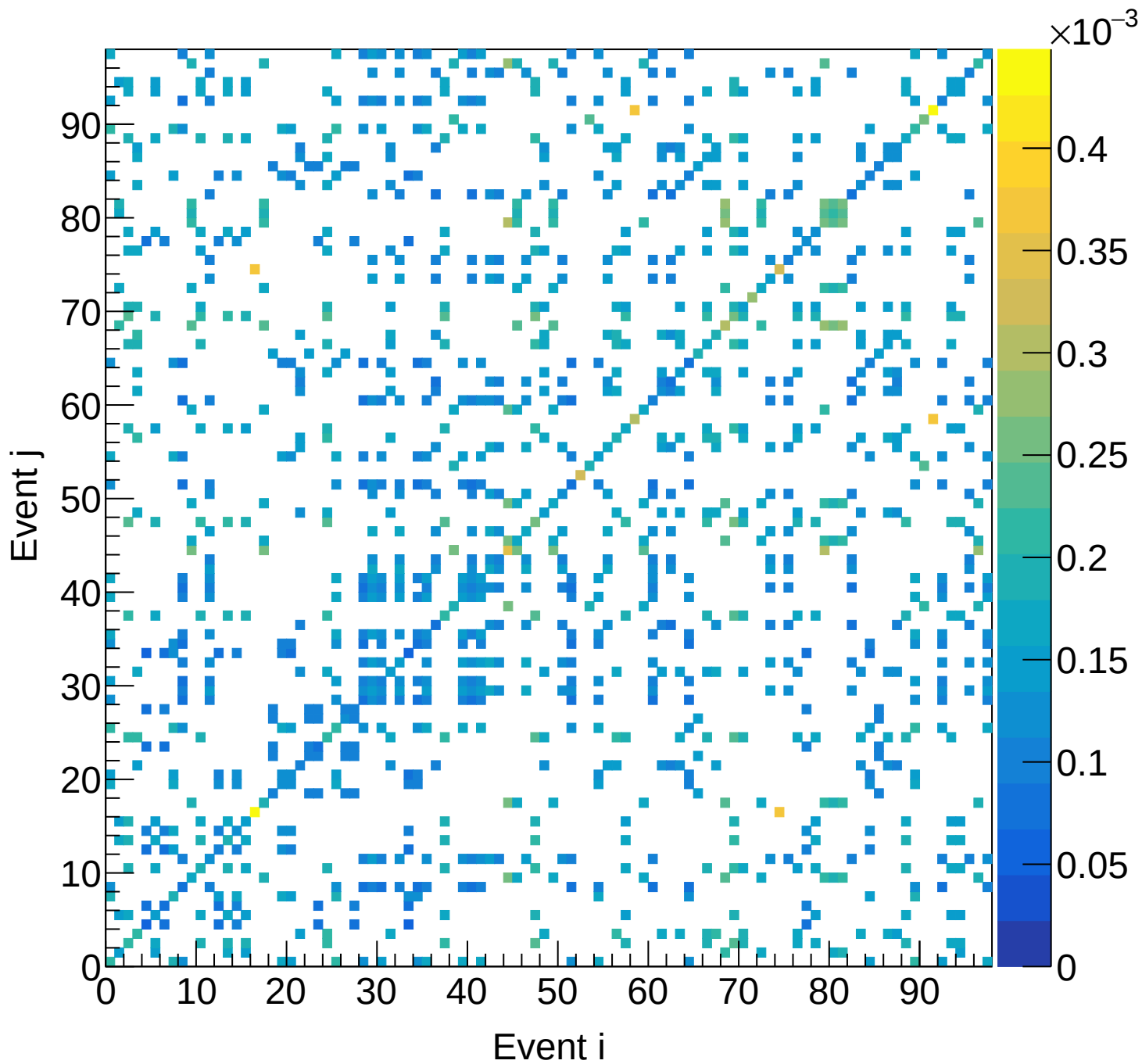
LH2 (total) Covariance | M: [4.2, 4.5) xF: [0.75, 0.80)
