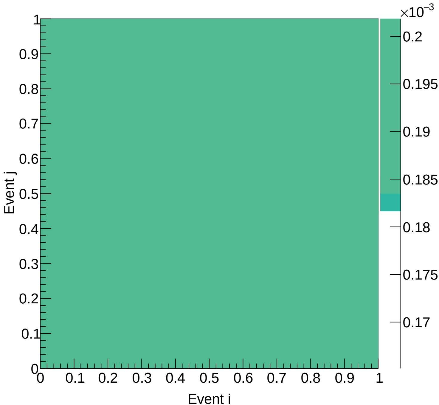
LH2 (total) Covariance | M: [6.9, 7.5) xF: [0.75, 0.80)
