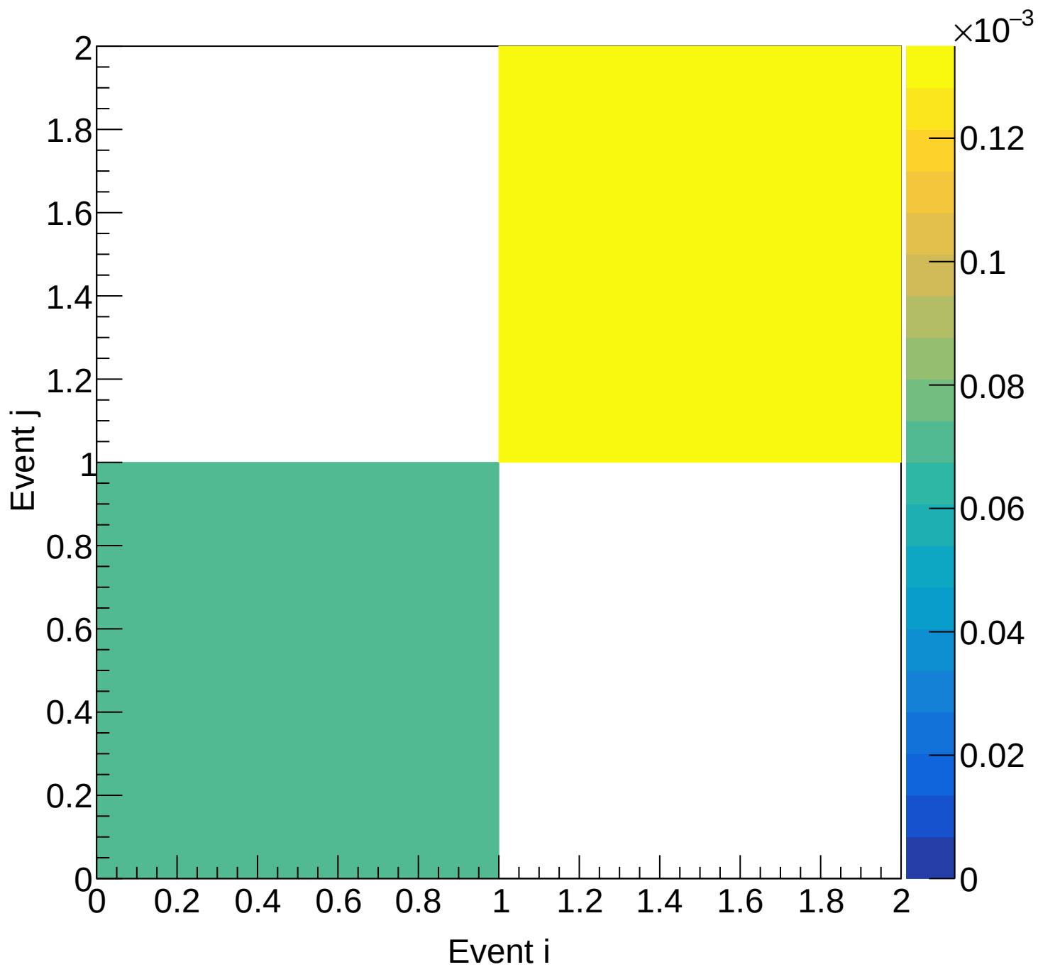
LH2 (total) Covariance | M: [7.5, 8.8) xF: [0.75, 0.80)
