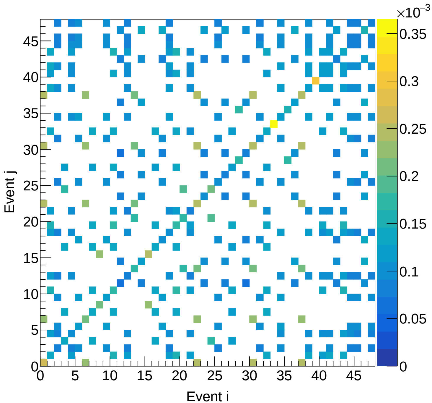
LH2 (total) Covariance | M: [4.5, 4.8) xF: [0.75, 0.80)
