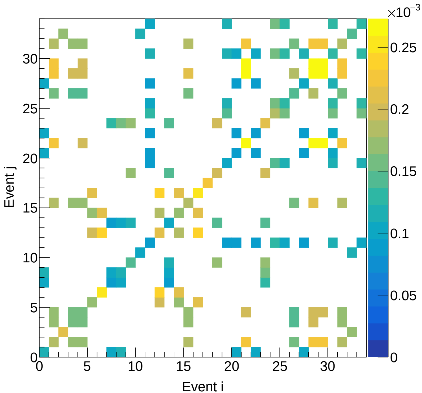
LH2 (total) Covariance | M: [4.8, 5.1) xF: [0.75, 0.80)
