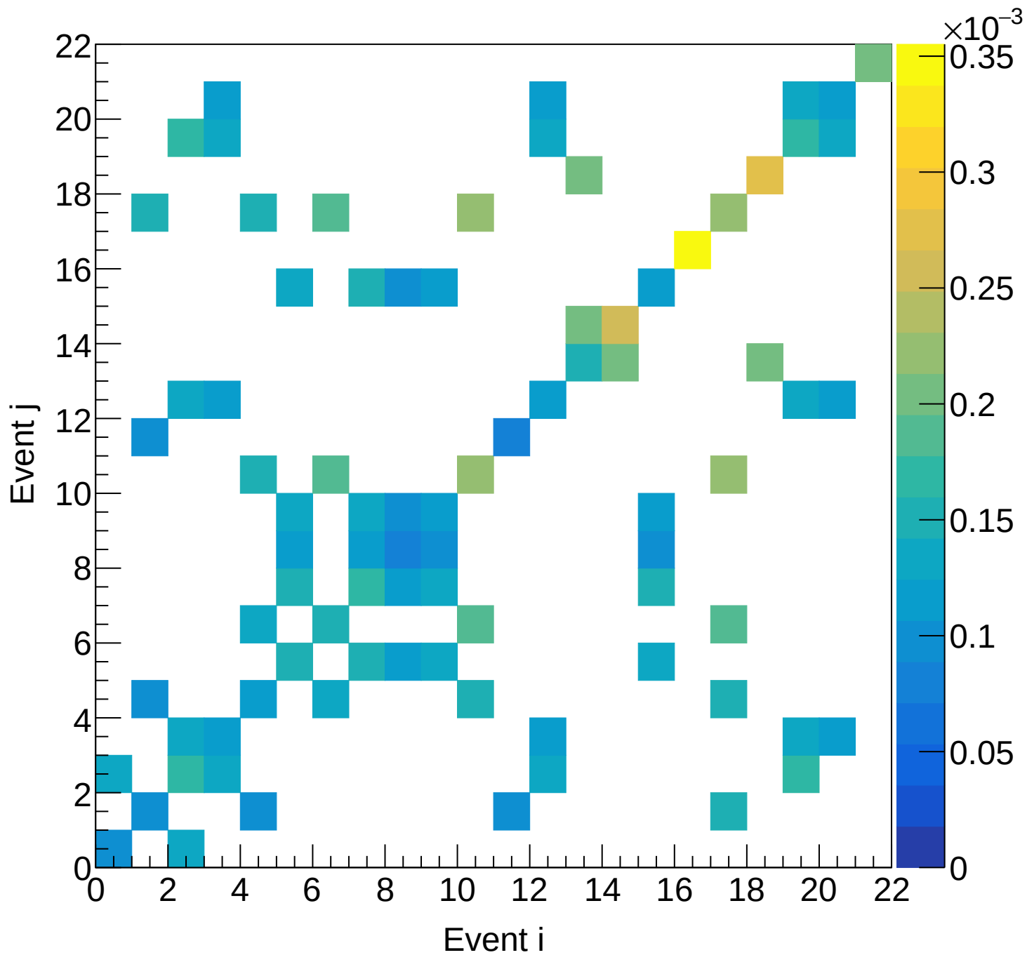
LH2 (total) Covariance | M: [5.1, 5.4) xF: [0.75, 0.80)
