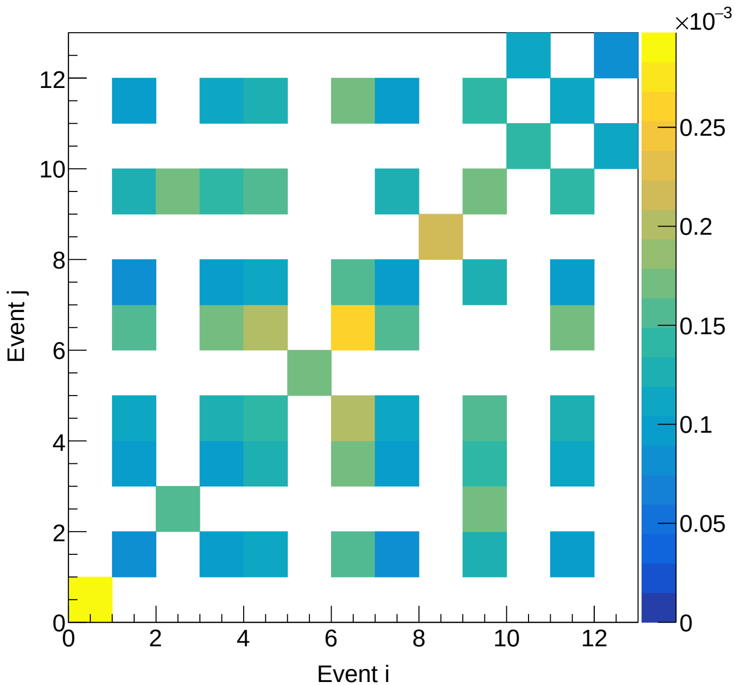
LH2 (total) Covariance | M: [6.0, 6.3) xF: [0.75, 0.80)
