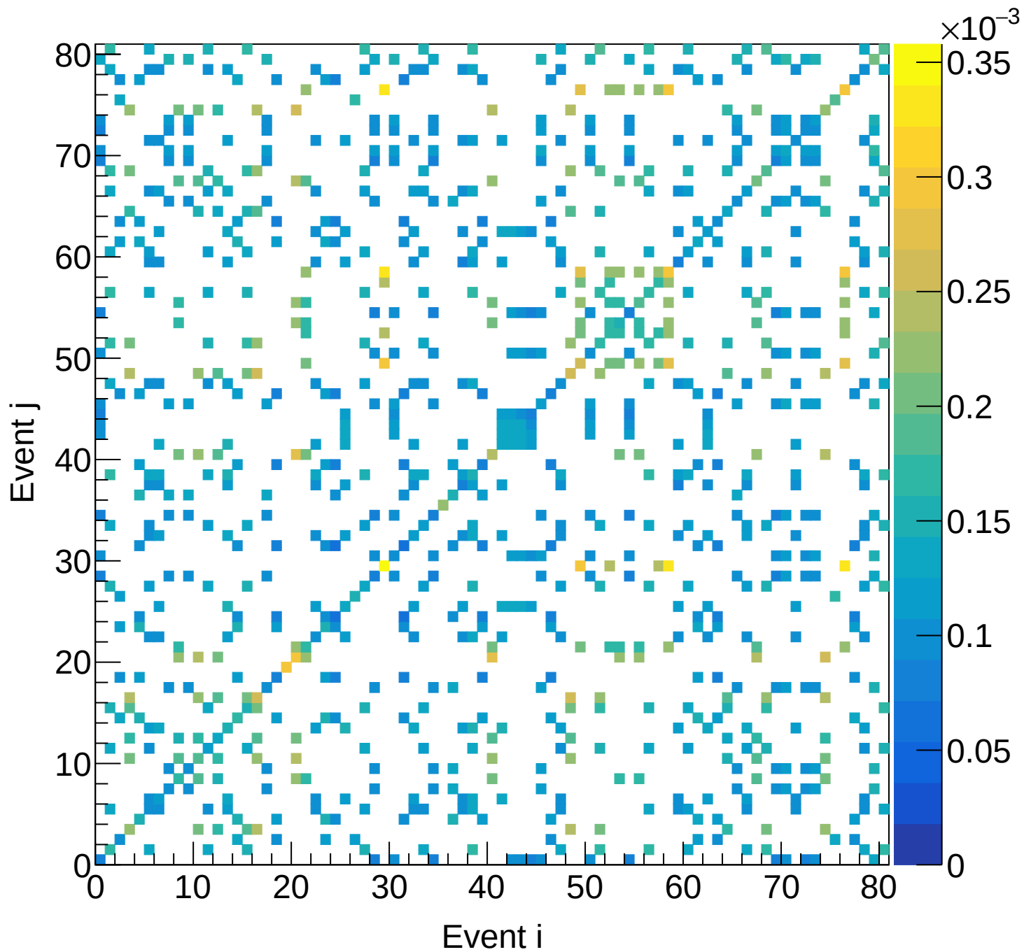
LH2 (total) Covariance | M: [3.9, 4.2) xF: [0.80, 0.85)
